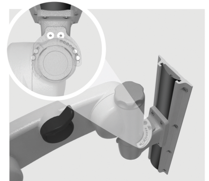
Rotational stop*
